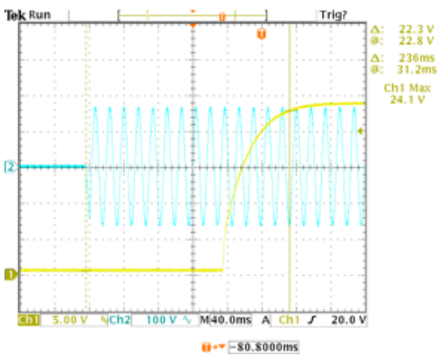
24V Turn-on delay, 115VAC
