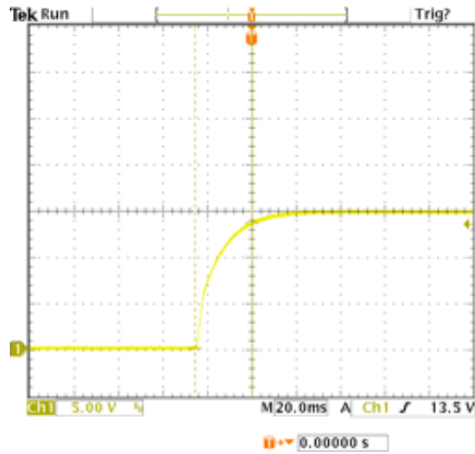
15V Rise Time
