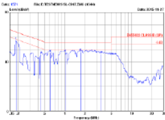
CISPR22 CLASS B QP 230V/50Hz 100% LOAD MARGIN: >7 dB
