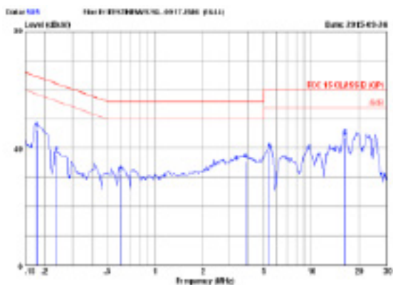
FCC15 CLASS B QP 100V/60Hz 100% LOAD MARGIN: >16 dB
