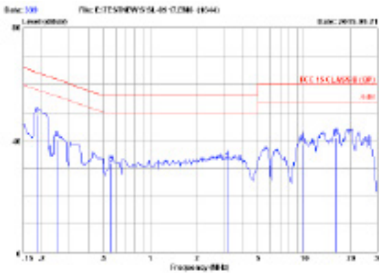
FCC15 CLASS B QP 100V/60Hz 100% LOAD MARGIN: >15 dB
