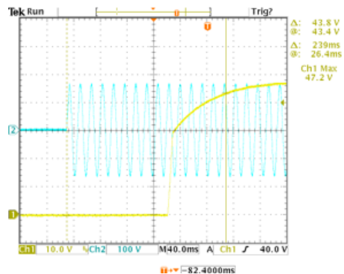
48V Turn-on delay, 115VAC
