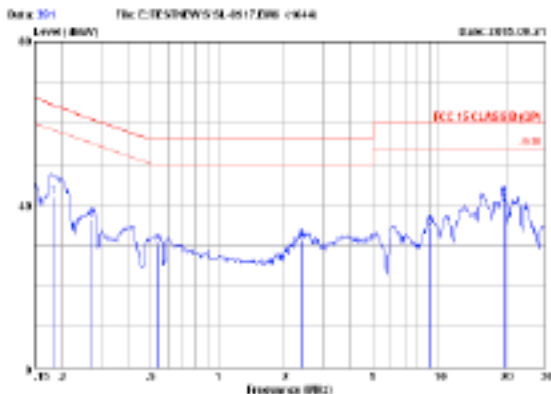
FCC15 CLASS B QP 100V/60Hz 100% LOAD MARGIN: >18 dB
