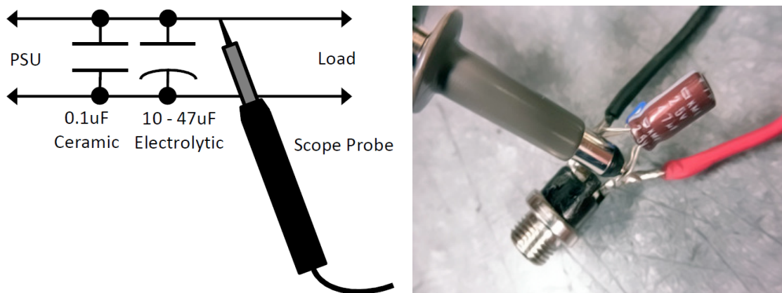
FIGURE 1: Noise measurement caps and probe with picture of the technique.
