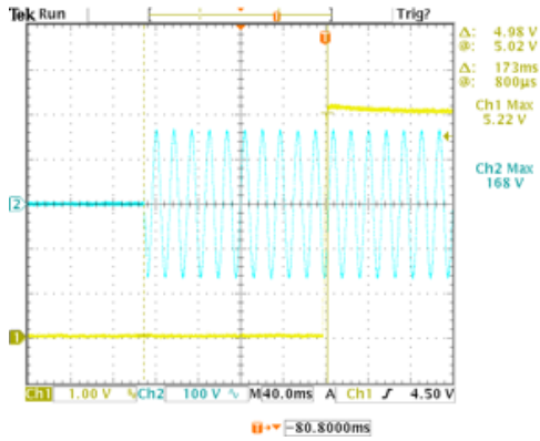
5V Turn-on delay, 115VAC
