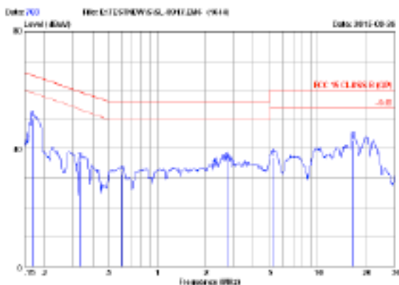
FCC15 CLASS B QP 100V/60Hz 100% LOAD MARGIN: >14 dB
