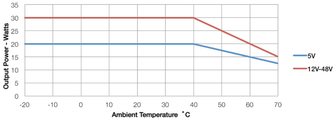
FIGURE 2: ME30 family derating curve.
