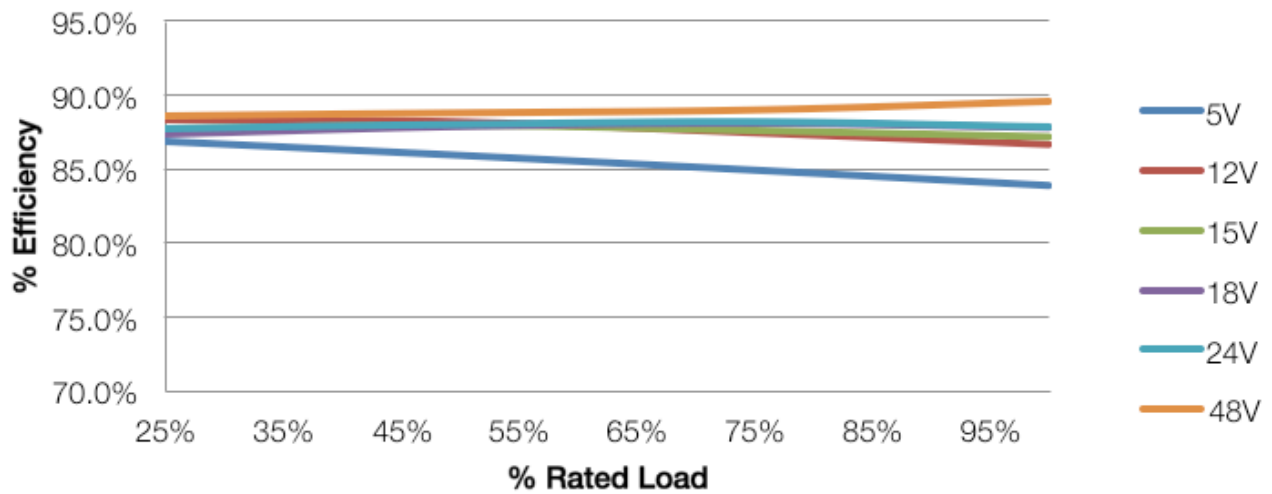
FIGURE 5: ME30 Series Efficiency @ 115VAC.
