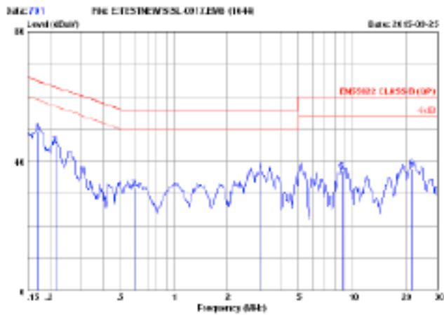
CISPR22 CLASS B QP 230V/50Hz 100% LOAD MARGIN: >15 dB
